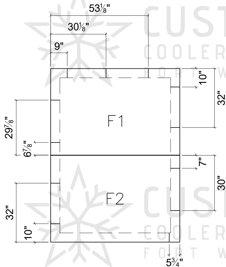
Pin Layout for Cam-Floors
